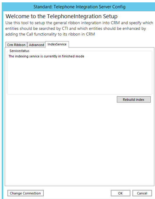
Figure 18: The IndexService-tab
