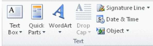
Figure 201: Field functions
