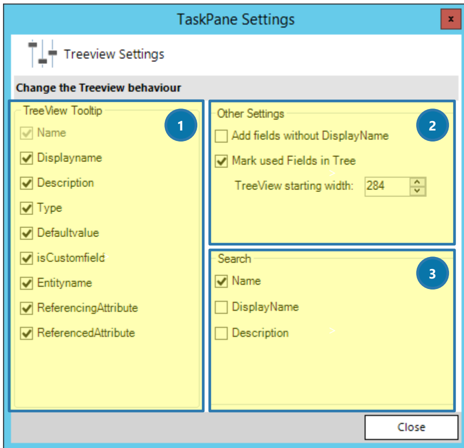
Figure 16: Taskpane settings
