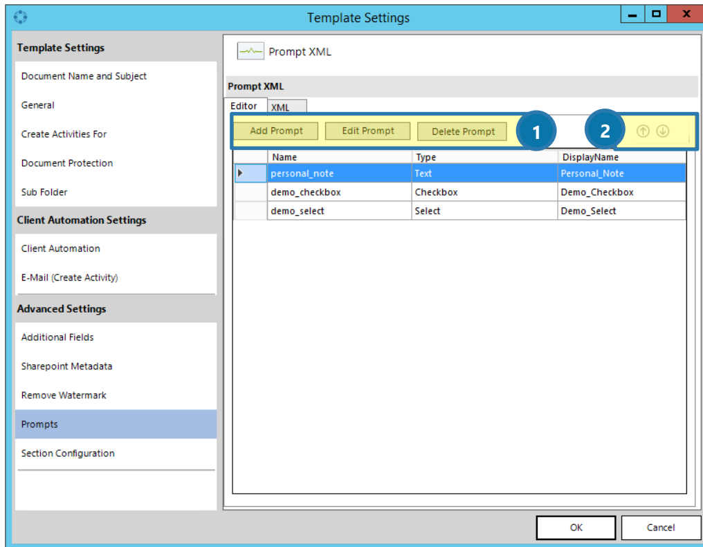
Figure 179: Prompt Editor
