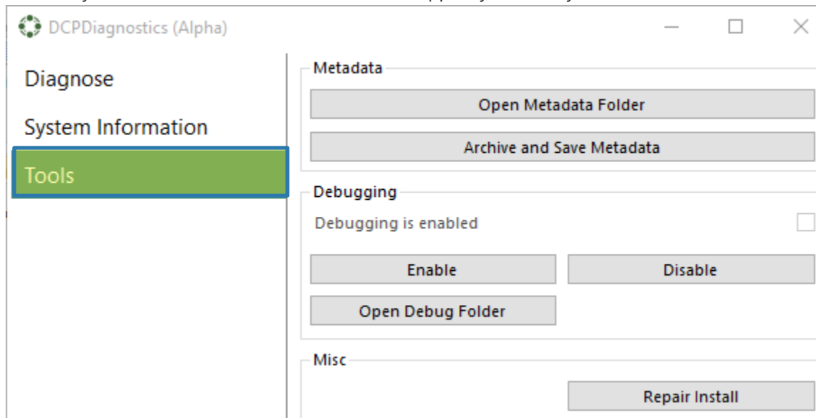
Figure 205: The Tools-tab
