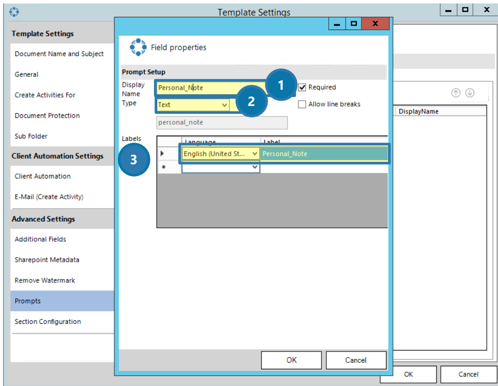
Figure 180: Prompt Setup
