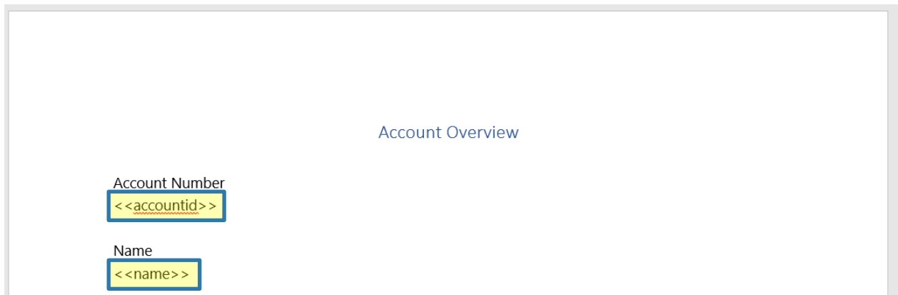
Figure 119: Insert fields
