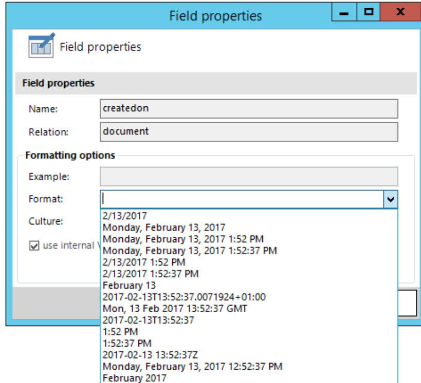
Figure 66: Insert Format
