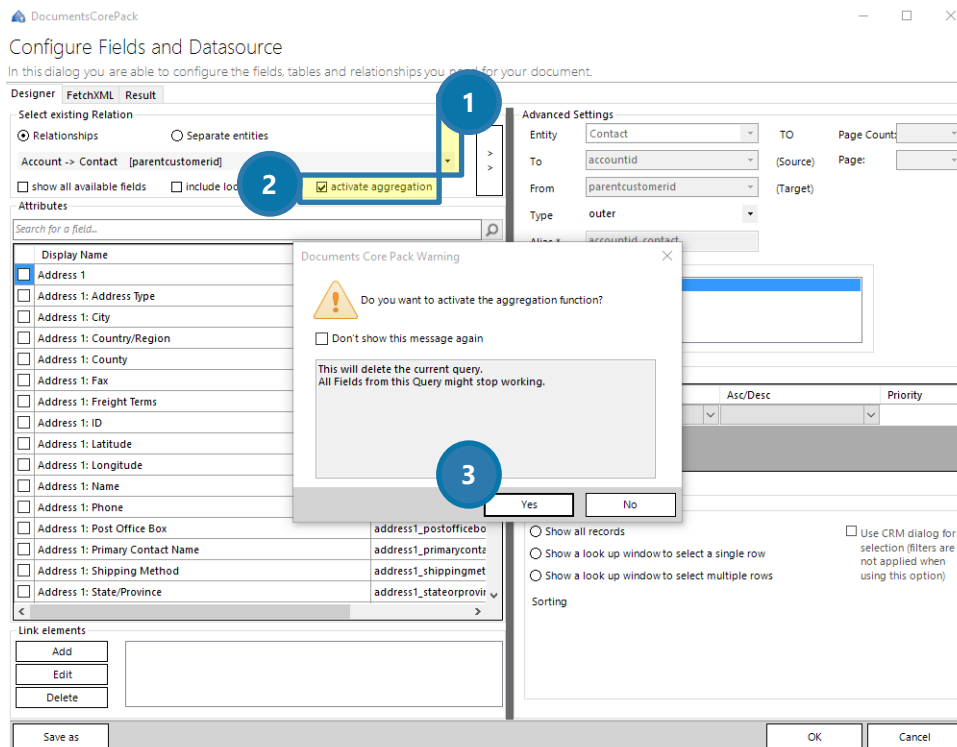
Figure 128: Activate aggregation
